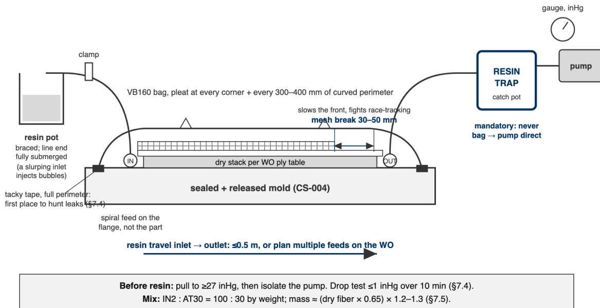
Figure 1: Figure 1. The full loop in section, pot to pump. The flow mesh stops 30–50 mm short of the outlet, the trap sits between bag and pump, and resin travel inlet to outlet stays at or under 0.5 m.
